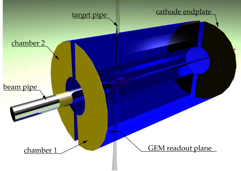
Figure 2: 3-D view of the PANDA TPC.
