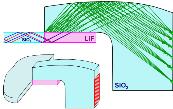
Fig. 4. Lightguide side view (inset 3D-visualisation) shown with a set of rays used for optimising the lightguide curvature. Reflections at the parallel front and back surfaces keep the light inside but do not affect the focussing properties.
