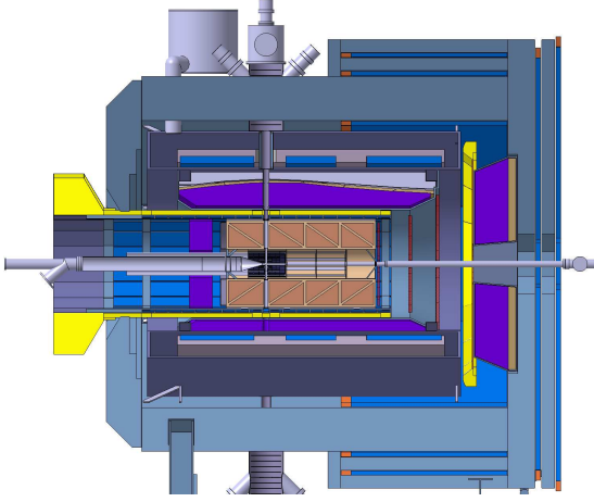
Fig. 1. \bar{P} ANDA target spectrometer. The Barrel and the Endcap DIRC detector positions are shown in light colour.
