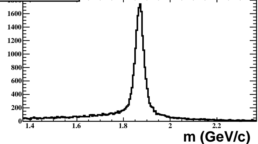
D - (K + π - π - ) invariant mass
