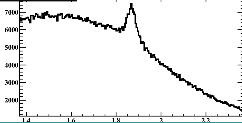
D + (K - π + π + ) invariant mass
