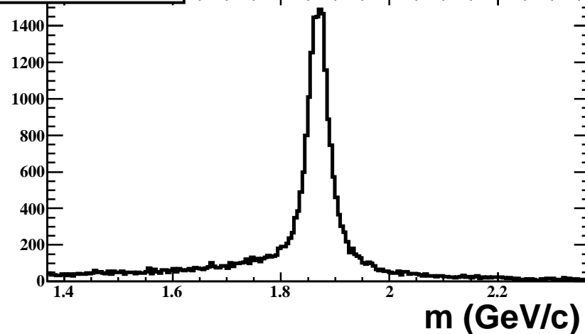
D + (K - π + π + ) invariant mass
